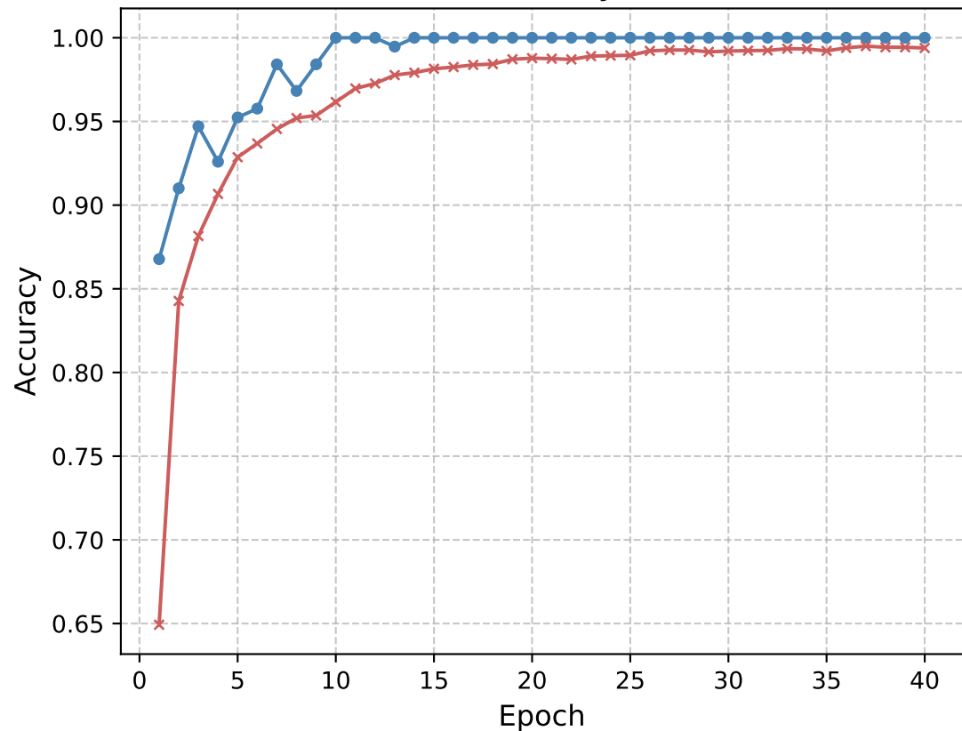
Accuracy
