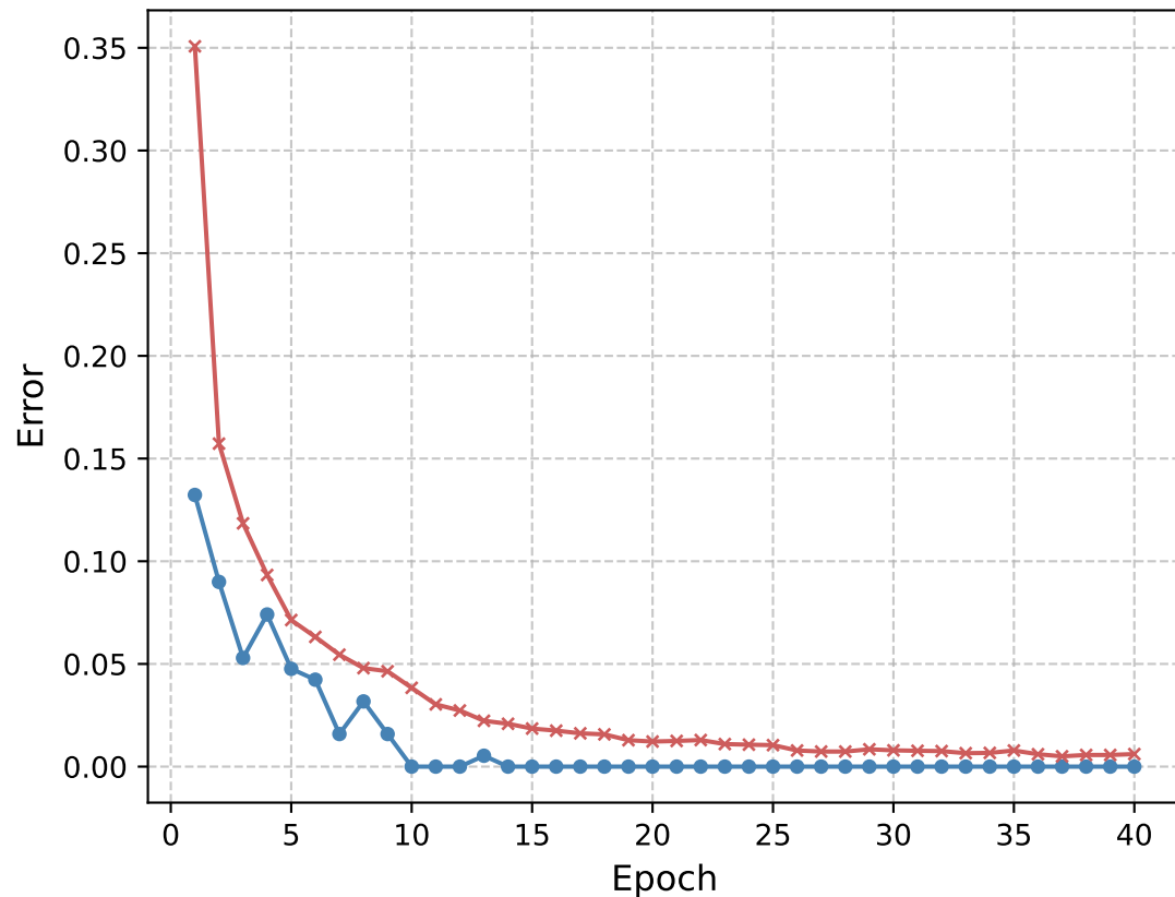
Error Rate
