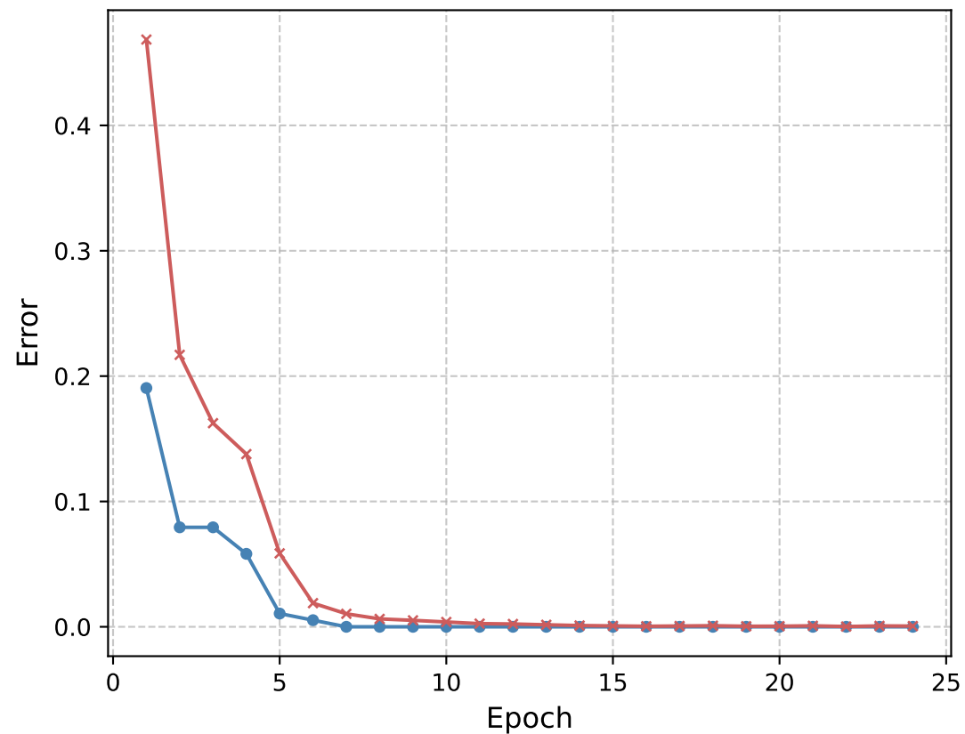
Error Rate
