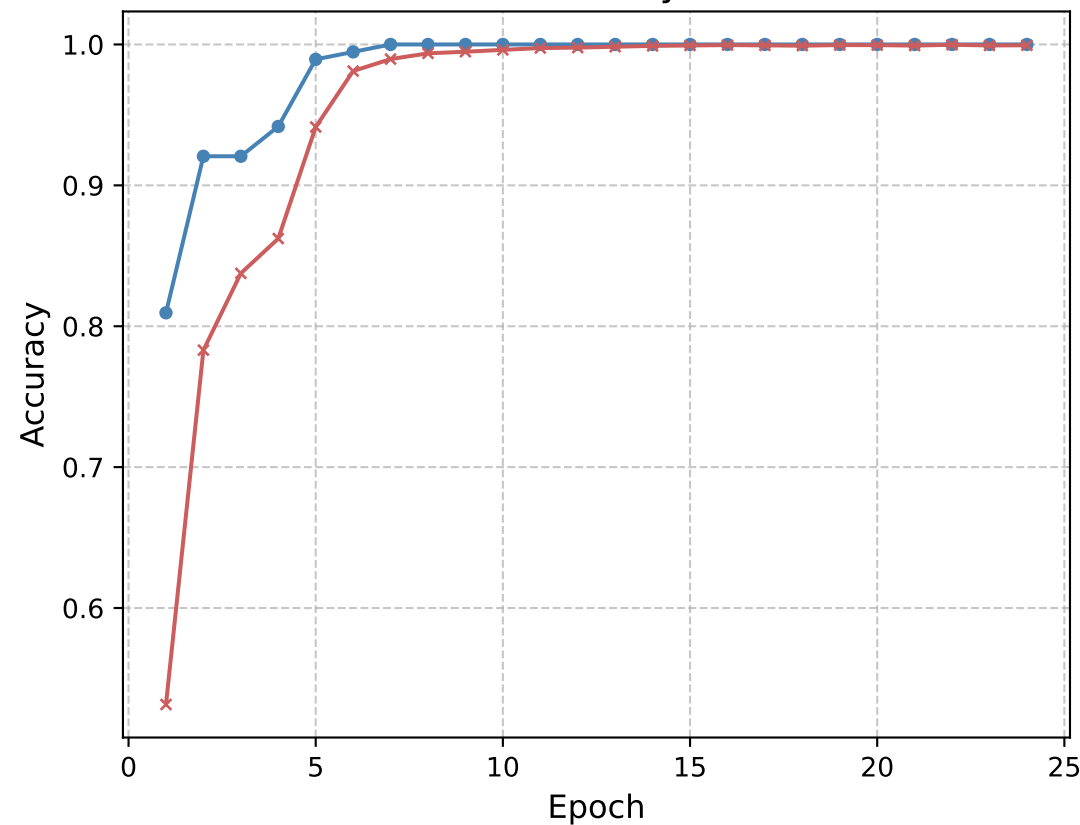
Accuracy
