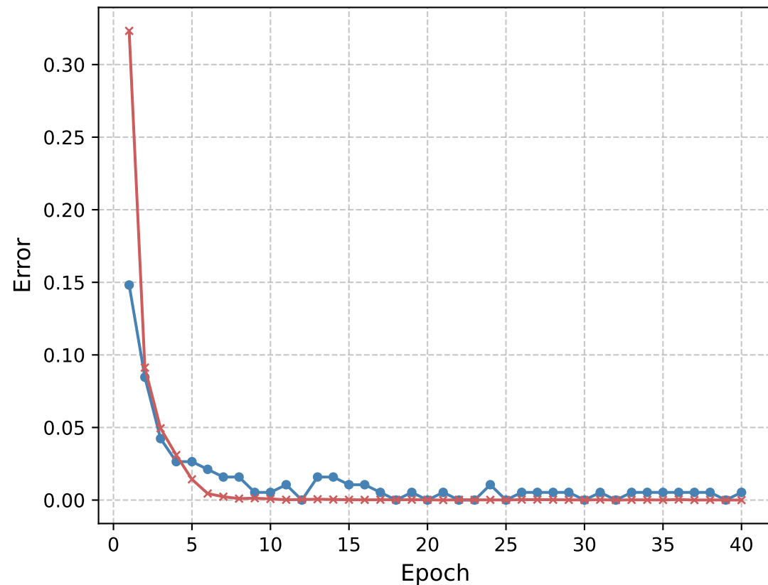
Error Rate
