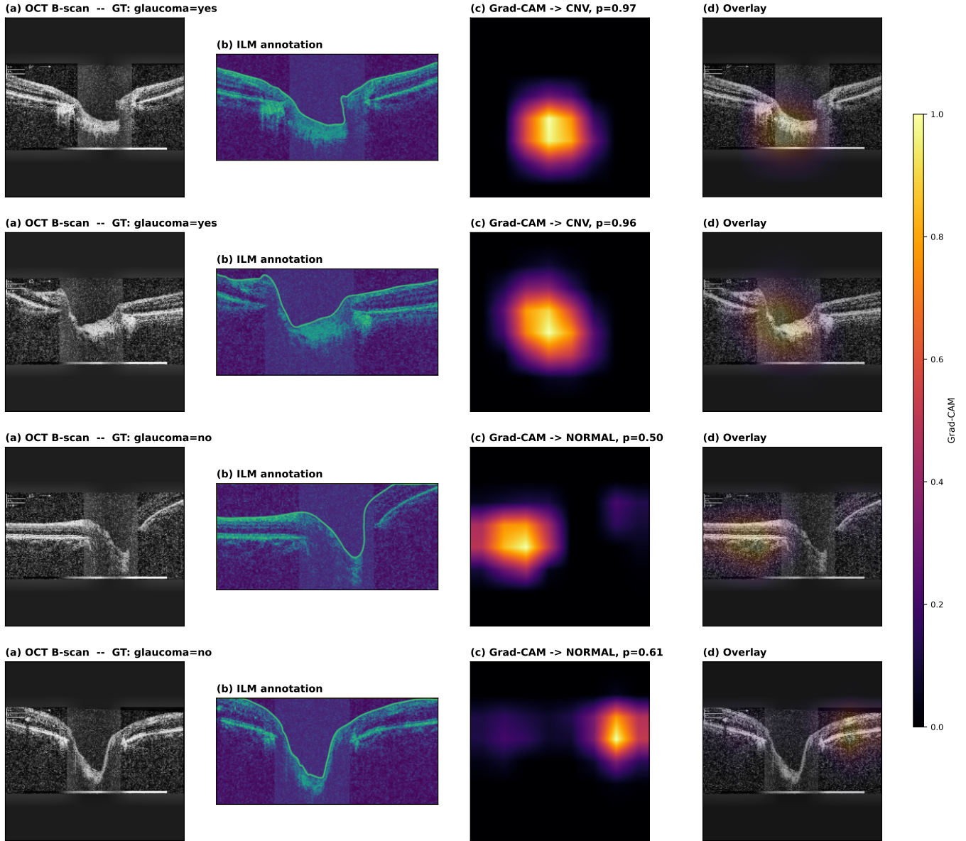
Figure 7: Qualitative paired-modality panel on the held-out ekacare glaucoma OCT cohort. (a) OCT B-scan with binary glaucoma label. (b) Cohort-provided ILM annotation. (c) Predicted-class Grad-CAM (Kermany class) on the same B-scan. (d) Overlay of (c) on (a). The activation overlays plausibly on annotated retinal layers despite the cross-cohort label-space mismatch.
