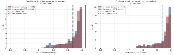
Figure 5: Confidence-shift histograms for the ResNet-18 baseline (left) and the ResNet-18 + SSM (right). Both panels show the max-softmax confidence density on the in-domain Kermany test ( n = 1,000 , blue) and the cross-cohort OCTID transfer ( n = 260 , red). The OOD mean is to the right of the ID mean for both models — the bare backbone is over-confident on inputs it has never seen, a behaviour quietly dangerous for clinical deployment. The SSM bottleneck does not fix the over-confidence but mildly attenuates the gap, consistent with the OOD-AUROC improvements in Table 7.
