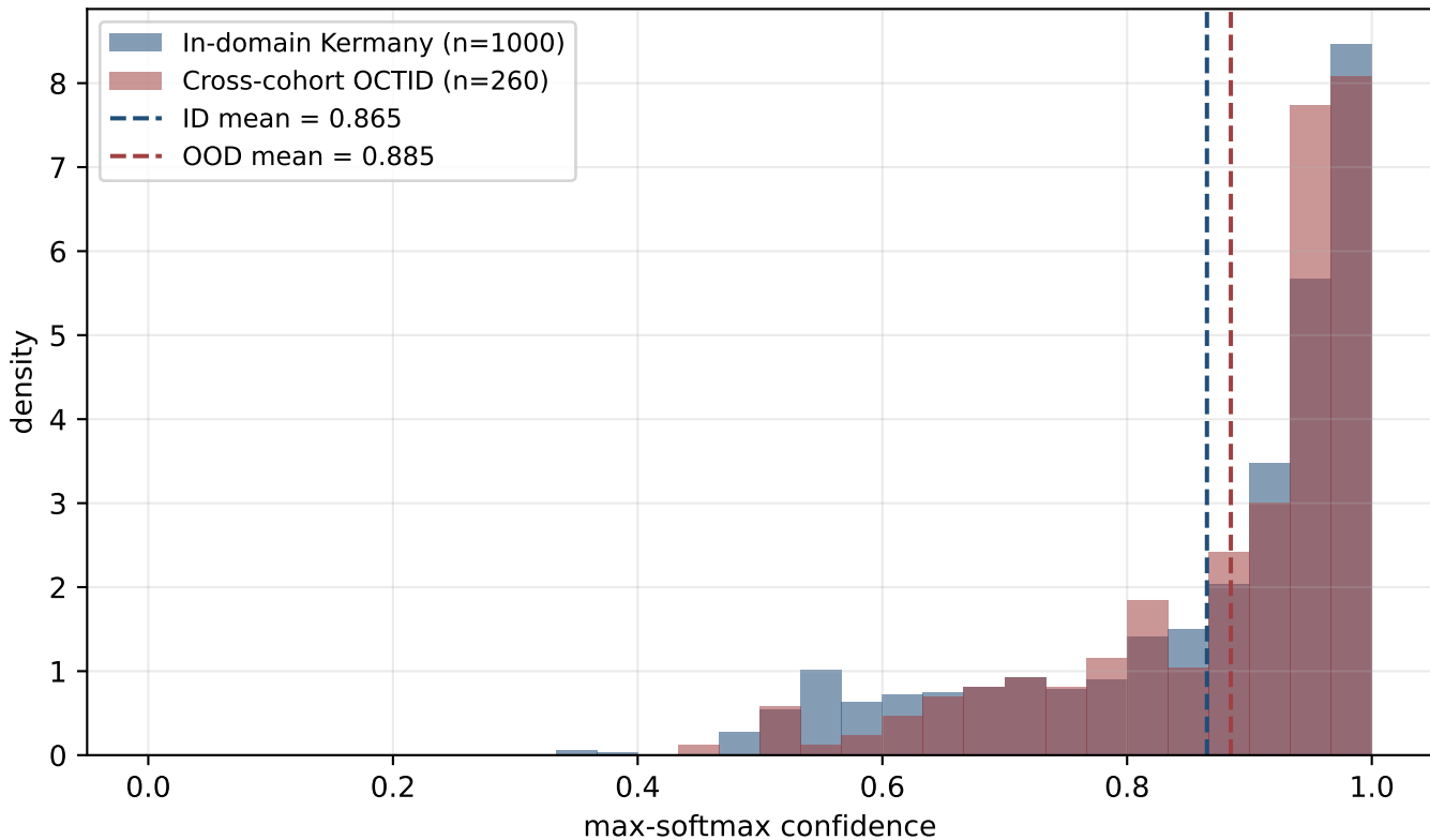
Confidence shift: in-domain vs. cross-cohort (SSM=False)
