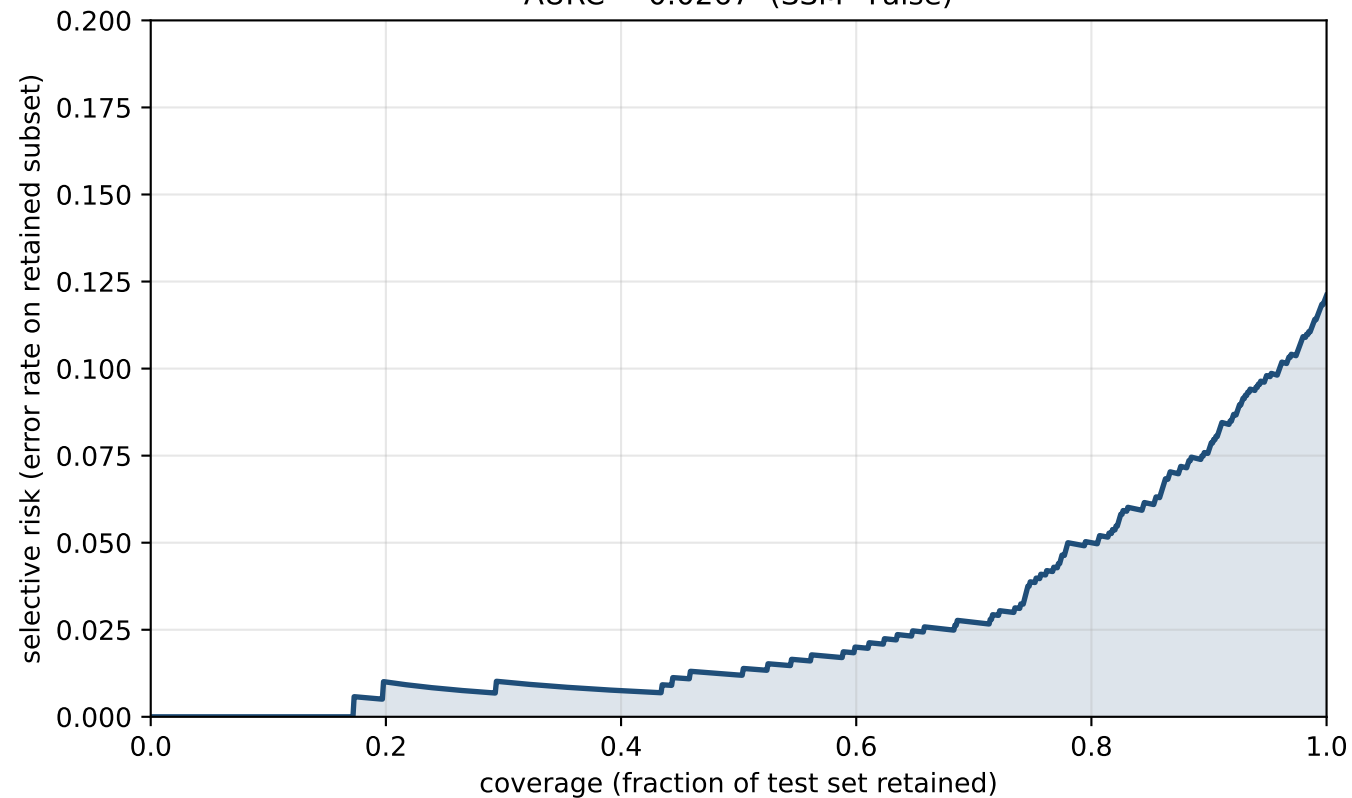
Risk-coverage curve on Germany 2017 test
