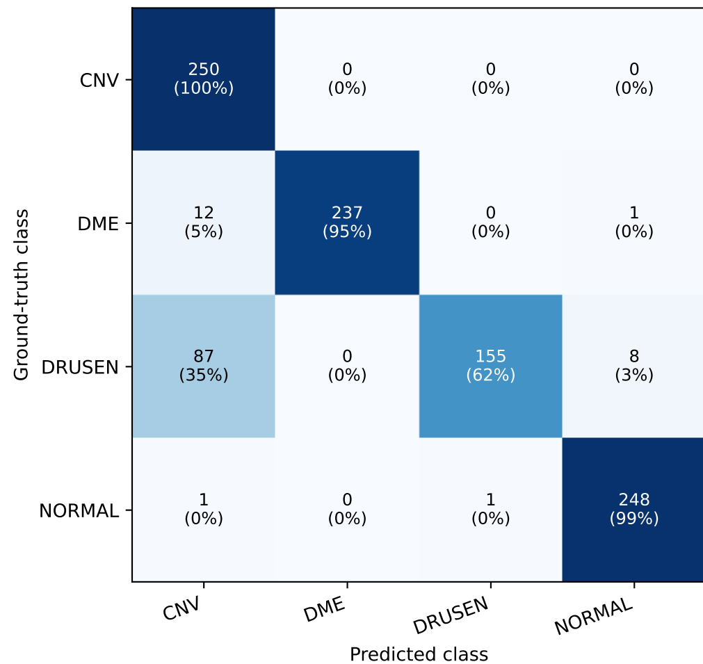
(a) Row-normalised confusion matrix
