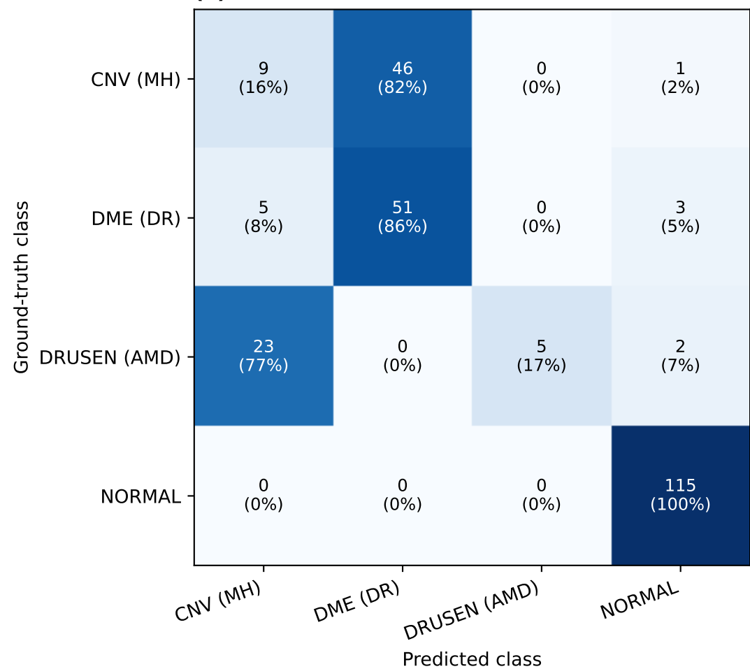
(a) Row-normalised confusion matrix
