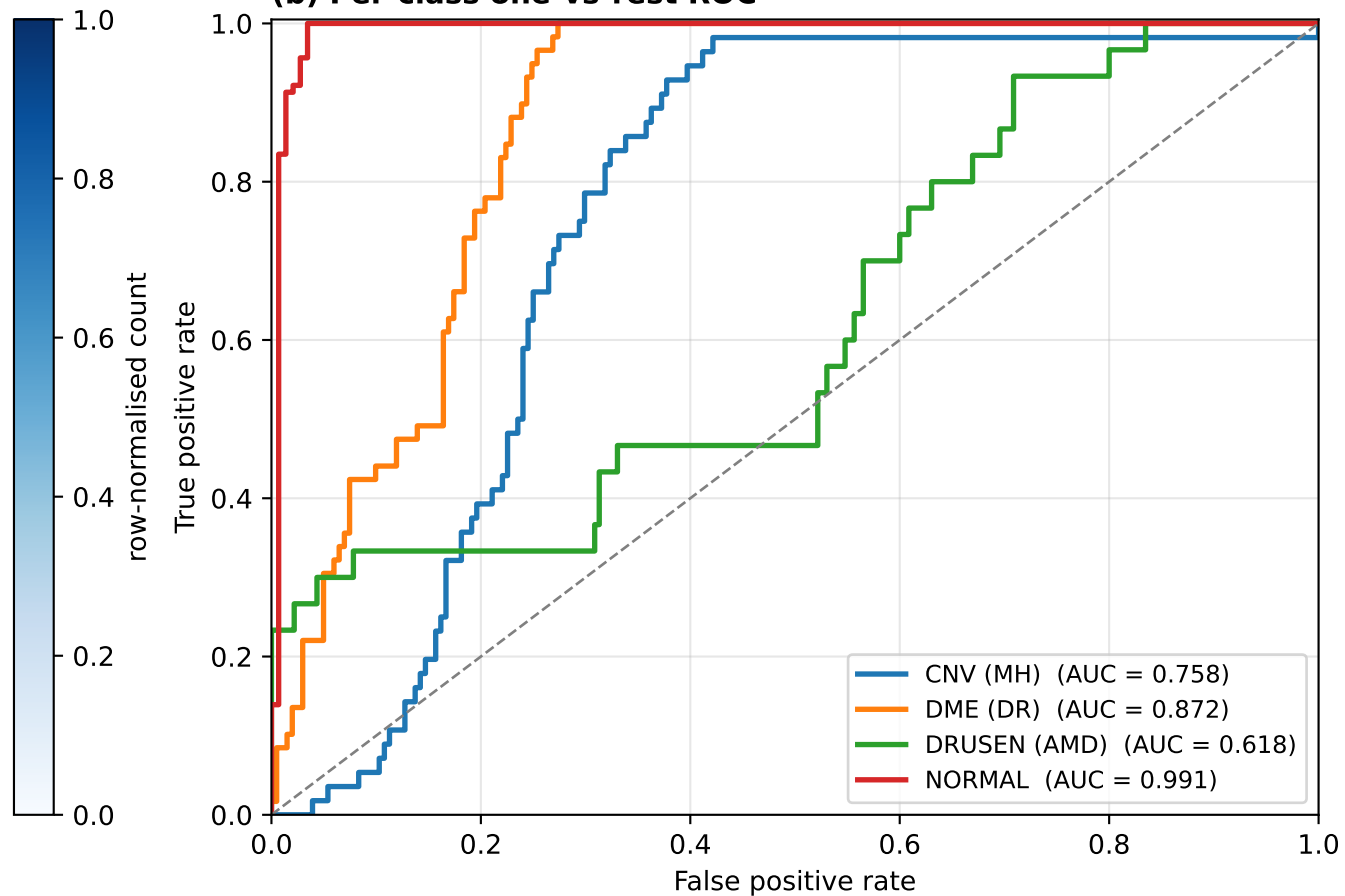
(b) Per-class one-vs-rest ROC
