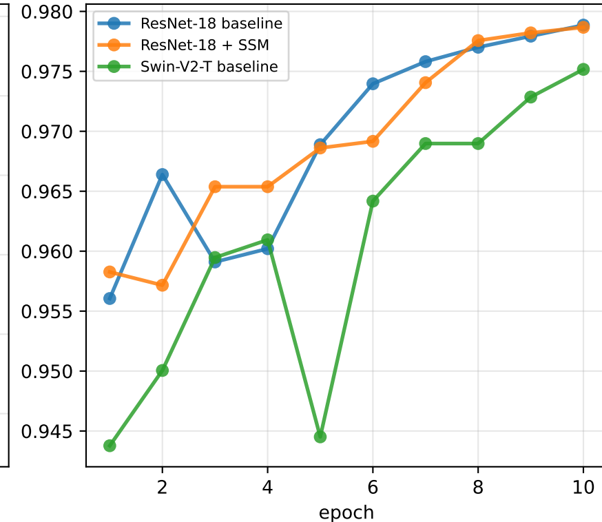
(b) Validation accuracy
