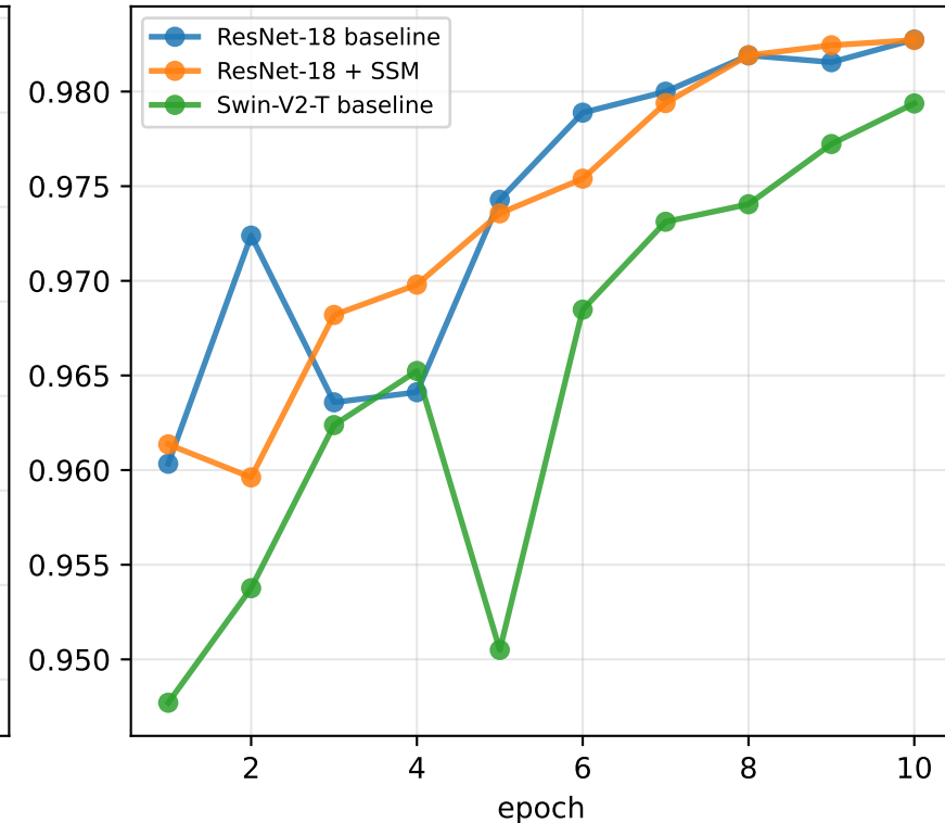
(c) Validation QWK
