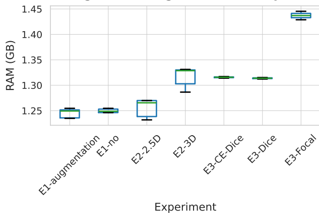
c) Average RAM Usage Across All Experiments
