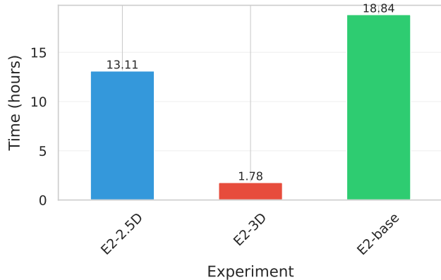
b) Average Training Time Until Convergence
