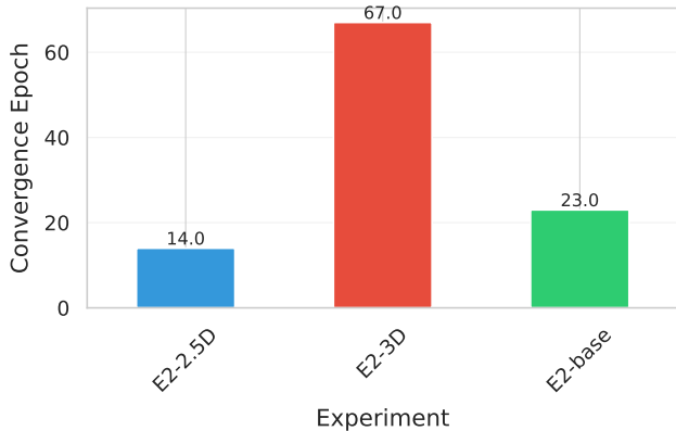
a) Average Convergence Epoch
