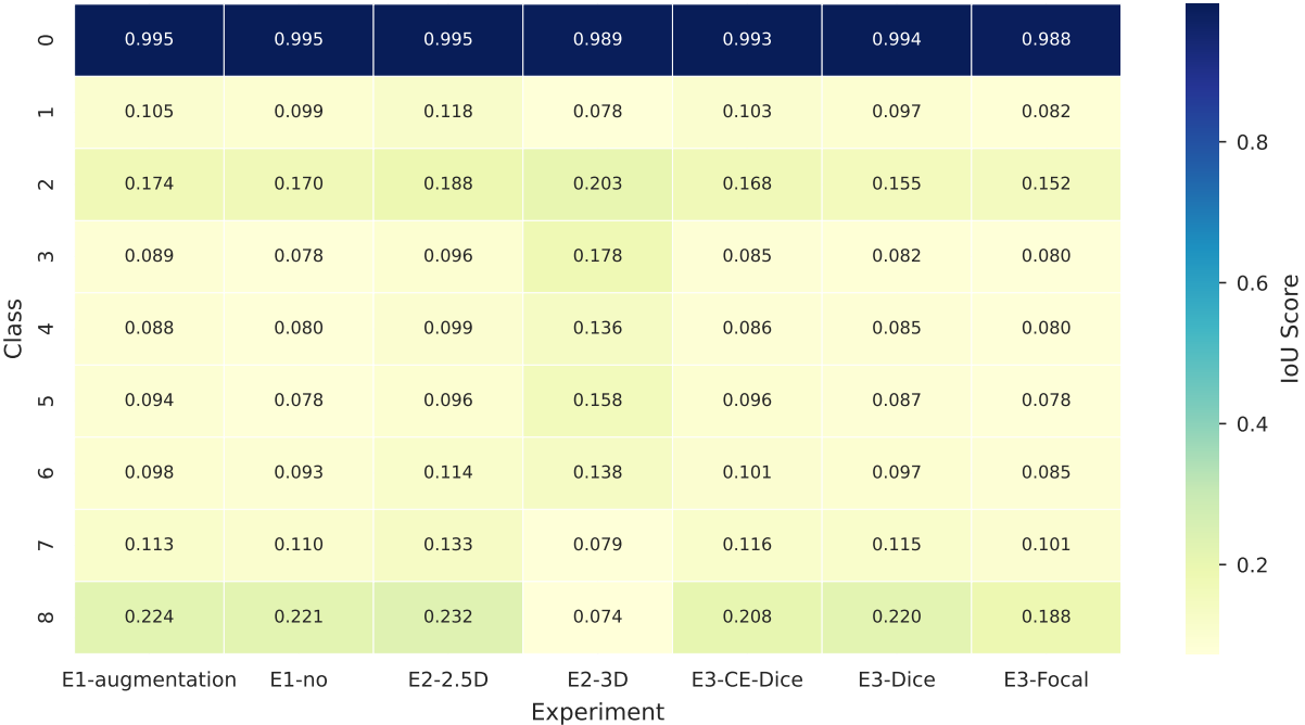
IoU Score Heatmap - All Experiments
