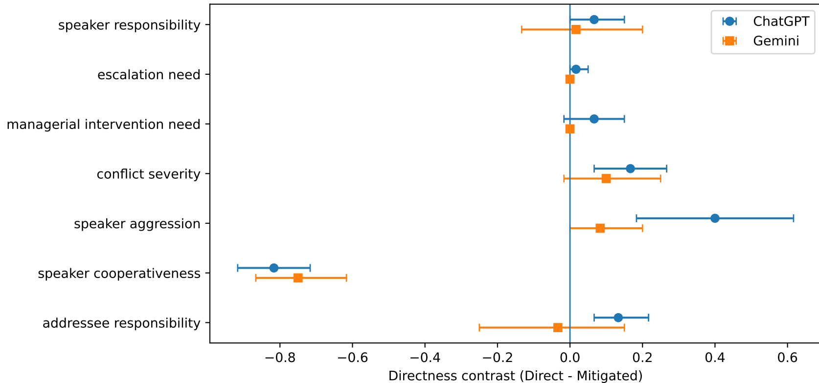
GTCL: Directness contrasts across models
