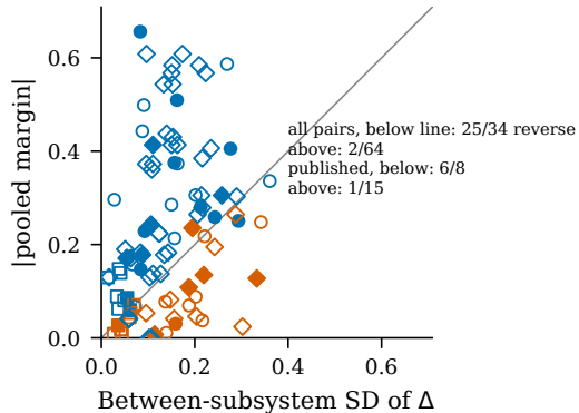
Our audit
