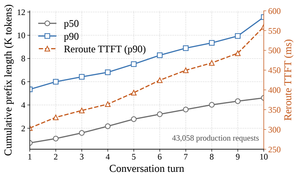
(a) Longer histories make rerouting slower
