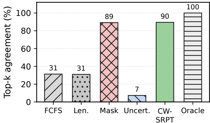
(b) Oracle batch-selection agreement
