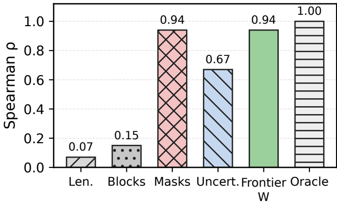
(a) Ranking accuracy against true remaining work
