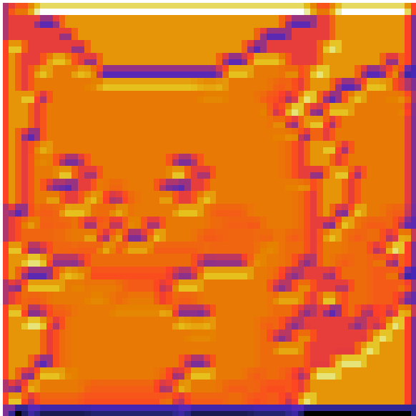
Convolution1: axis0
