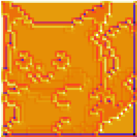
Convolution1: axis1
