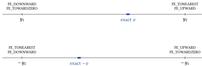
Fig. 15. What each mode returns when the exact result v falls between the representable neighbors y_1 < y_2 , shown for v and for -v . Round to nearest ignores the sign. The directed modes do not: round toward zero picks the lower neighbor for positive values and the upper neighbor for negative ones.
