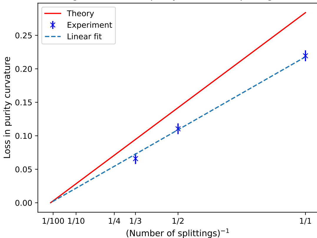
Small-angle curvature of purity vs. inverse splitting of rotation
