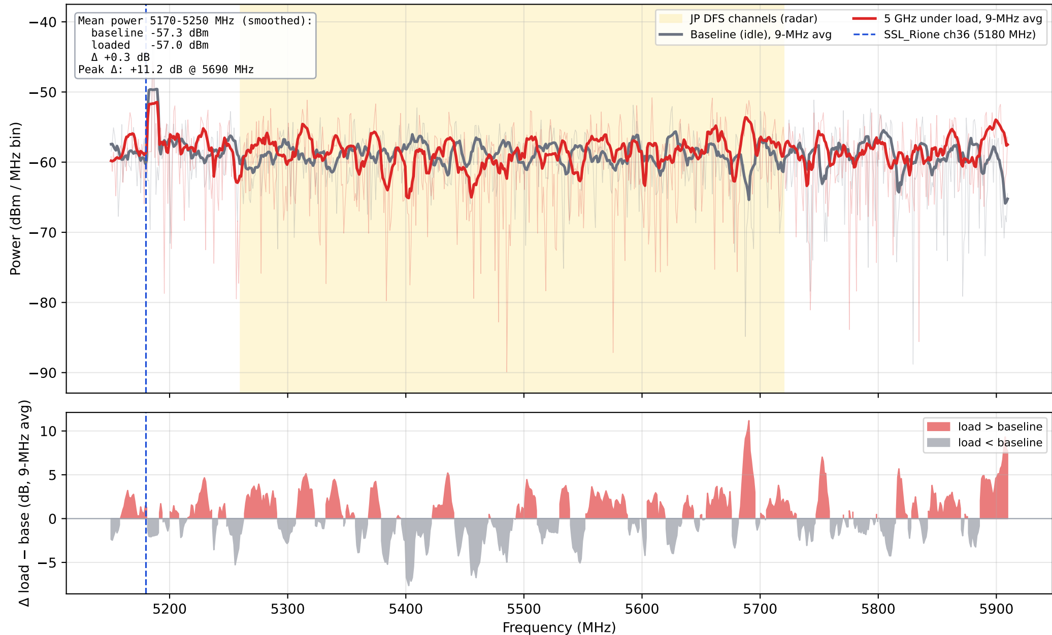
5 GHz spectrum: idle baseline vs. network under load (HackRF sweep, 1 MHz bins, 2 passes)
