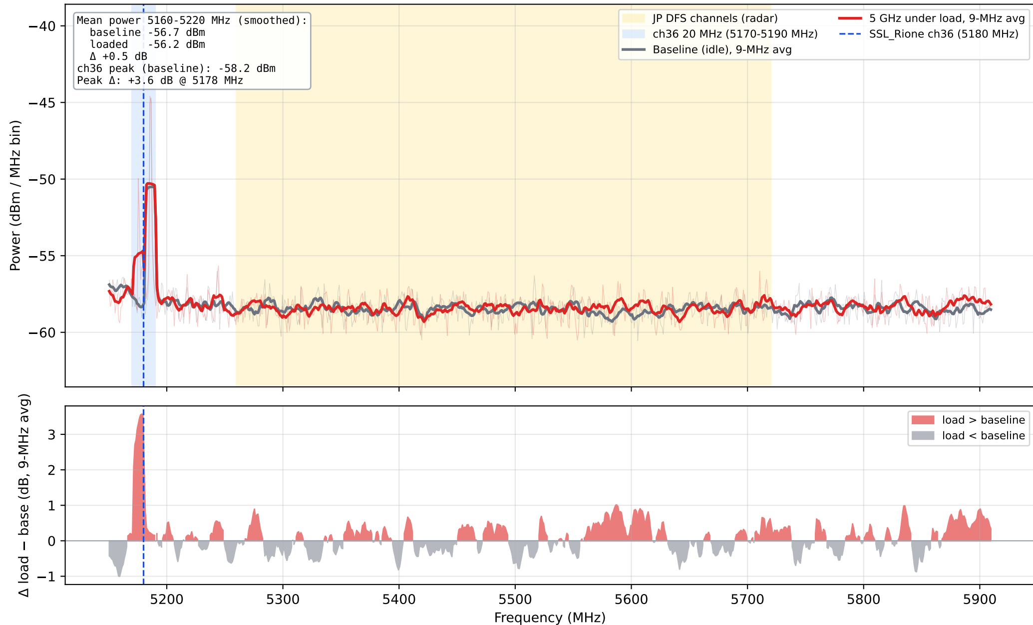
5 GHz spectrum (full band): idle baseline vs. network under load (HackRF sweep, 1 MHz bins, 50 passes)
