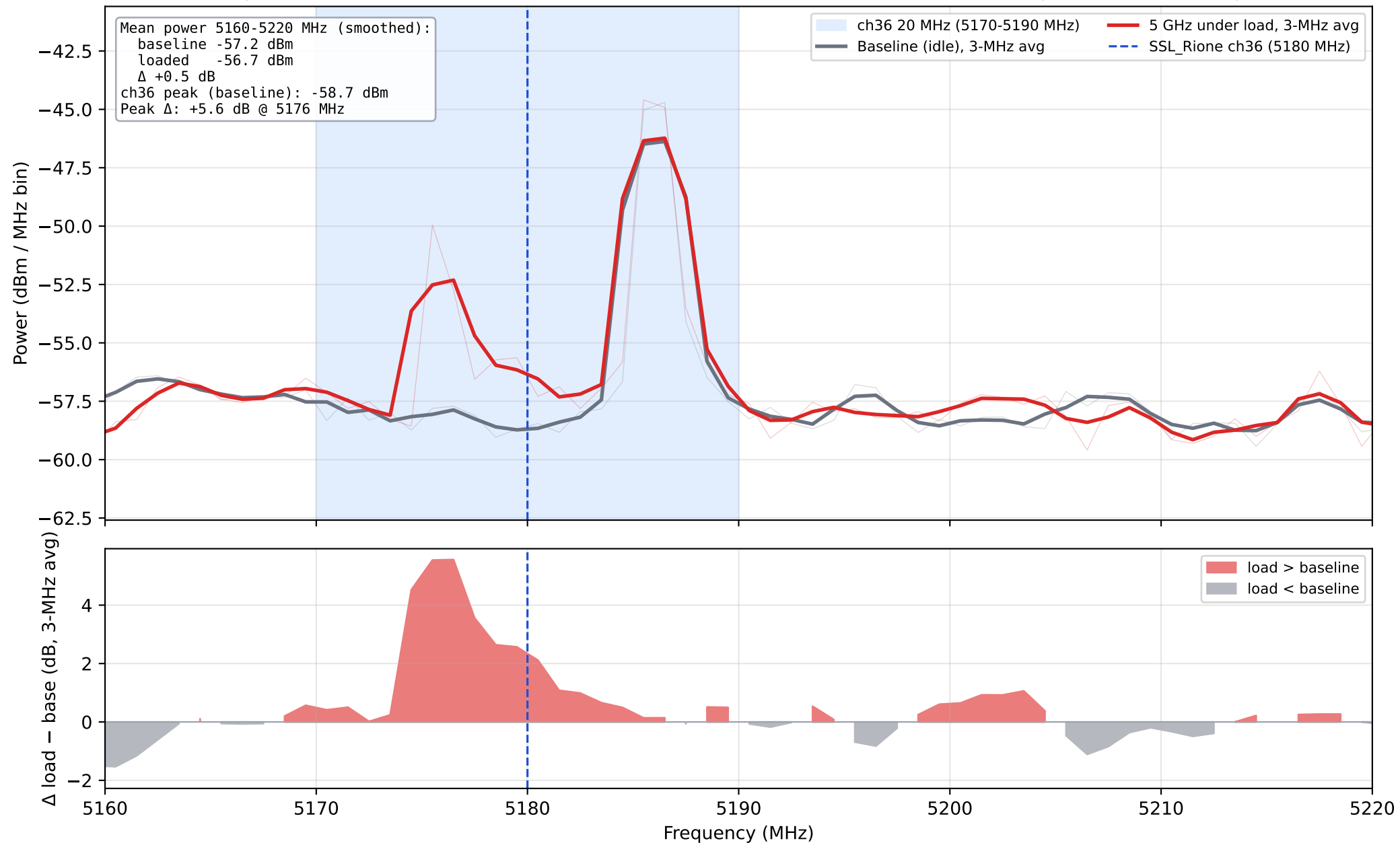
5 GHz spectrum (ch36 zoom): idle baseline vs. network under load (HackRF sweep, 1 MHz bins, 50 passes)
