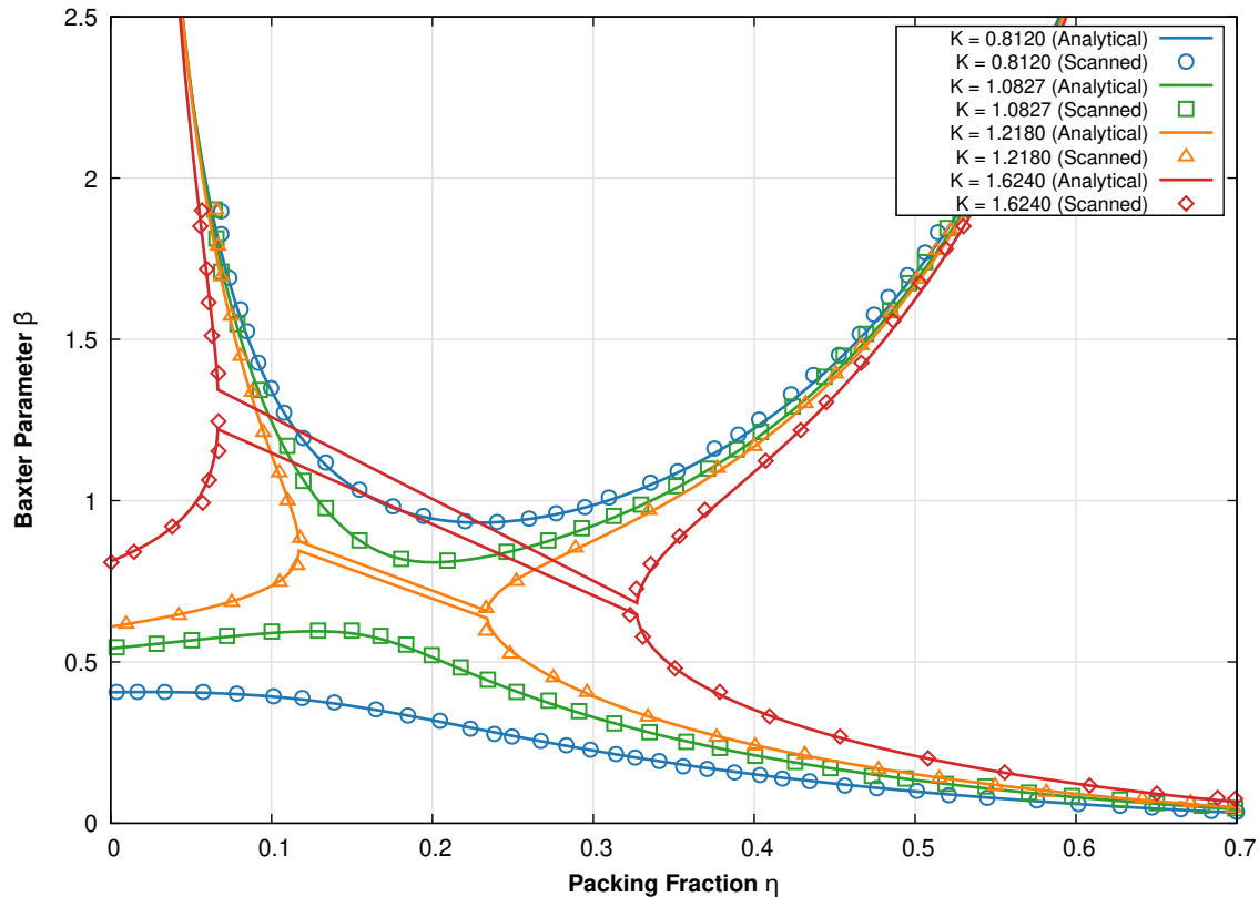
Cummings Smith (1979) - Fig. 1: Parameter \beta vs Density \eta ( \xi = 2 )
