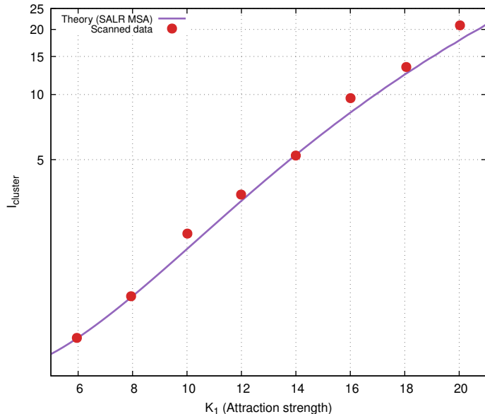
FIG. 1: Cluster Peak in Structure Factor S(Q) and Peak Intensity I_{\text{cluster}}
