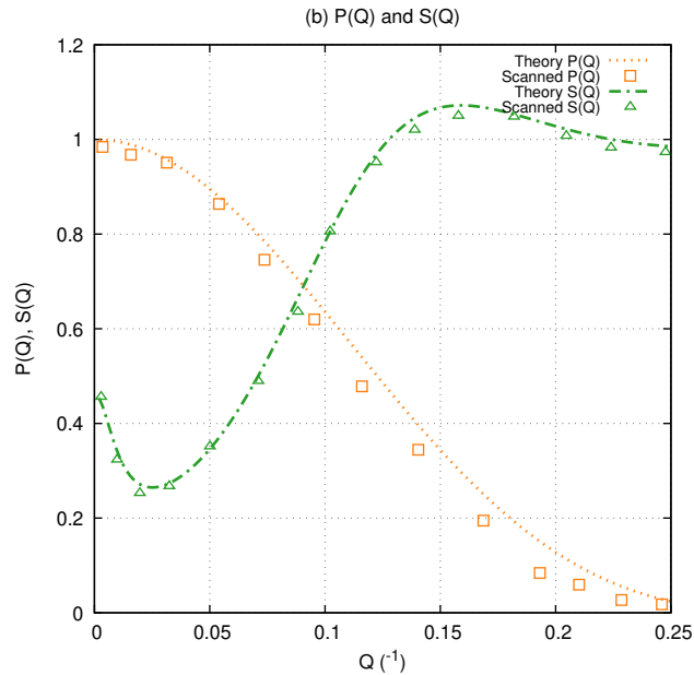
FIG. 11: Application to SANS of Cytochrome C (10.18 wt%)
