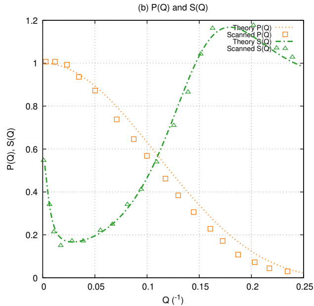
FIG. 12: Application to SANS of Cytochrome C (20.40 wt%)
