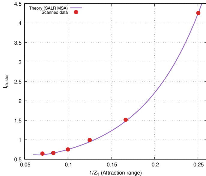
FIG. 2: Effect of Attraction Range 1/Z_1 on S(Q) and I_{\text{cluster}}
