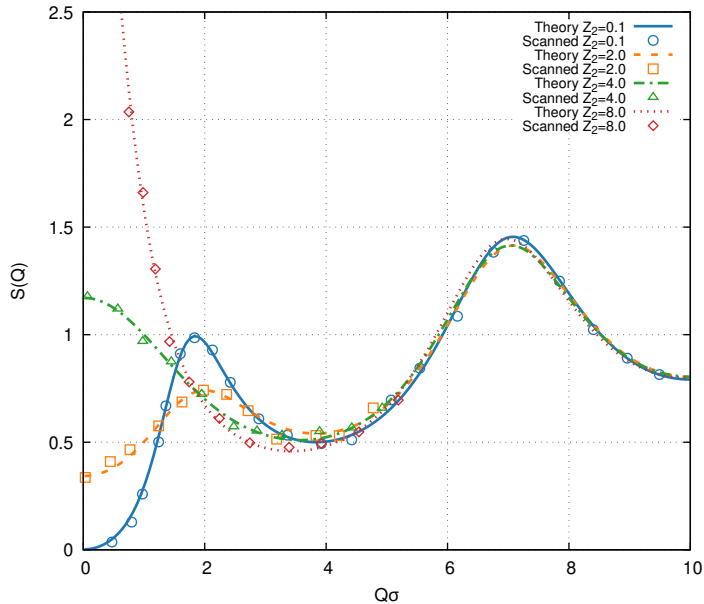
FIG. 4: Effect of Repulsion Range 1/Z_2 on S(Q) and I_{\text{cluster}}
