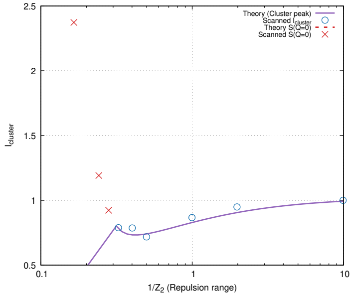
FIG. 4: Effect of Repulsion Range 1/Z_2 on S(Q) and I_{\text{cluster}}
