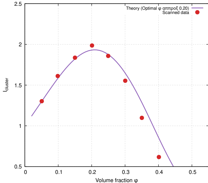
FIG. 5: Volume Fraction Dependence of S(Q) and I_{\text{cluster}}
