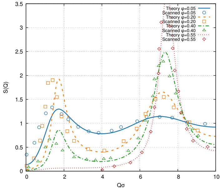
FIG. 5: Volume Fraction Dependence of S(Q) and I_{\text{cluster}}
