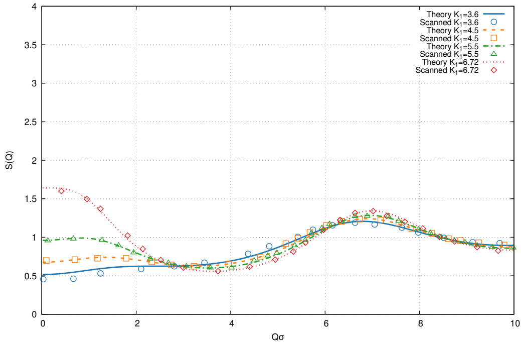
FIG. 7: Static Structure Factor S(Q) at \varphi=0.15 for Indicated Attraction K_1
