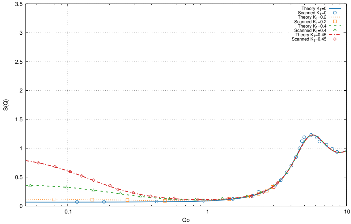
FIG. 9: S(Q) for Short-Range Repulsion Long-Range Attraction ( \phi=0.20 , Z_1=0.5 , K_2=-2 , Z_2=2 )
