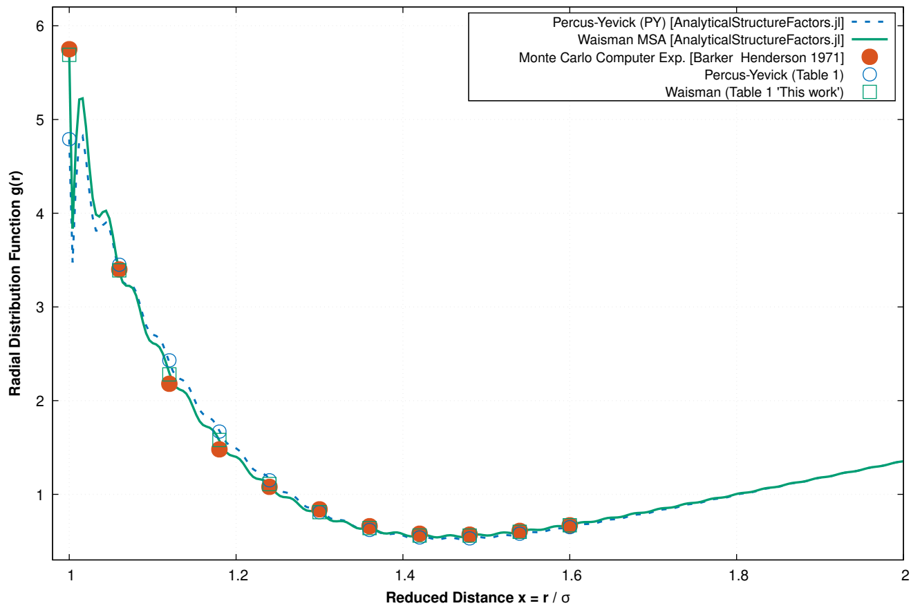
Hard Sphere Fluid at High Density ( \eta = 0.49 ): Radial Distribution Function g(r) Validation against Waisman (1973) Mol. Phys. 25, 45-48
