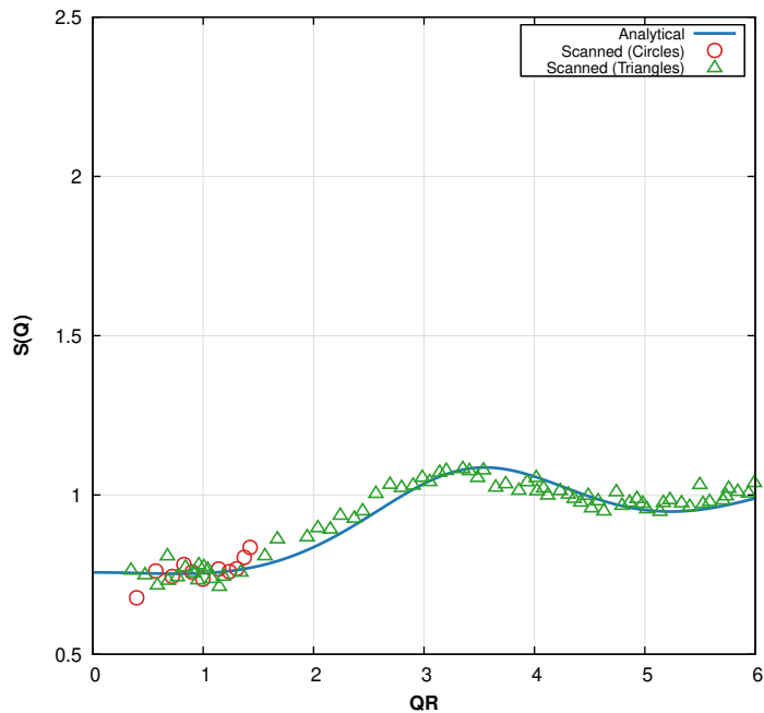
(b) Homogeneous S(Q) ( \eta=0.0931 , \tau=0.3653 )
