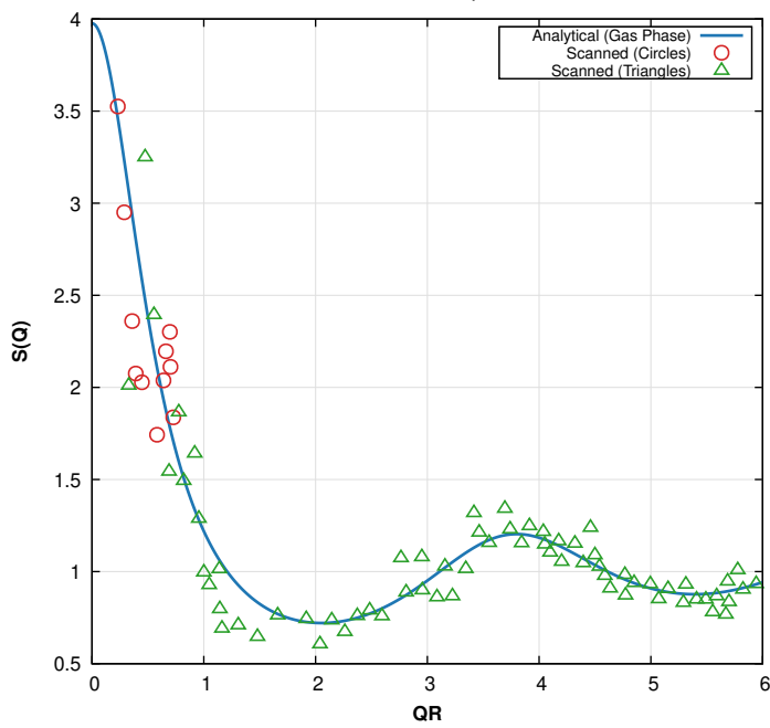
(c) Coexistence Gas S(Q) ( \eta=0.0581 , \tau=0.0923 )
