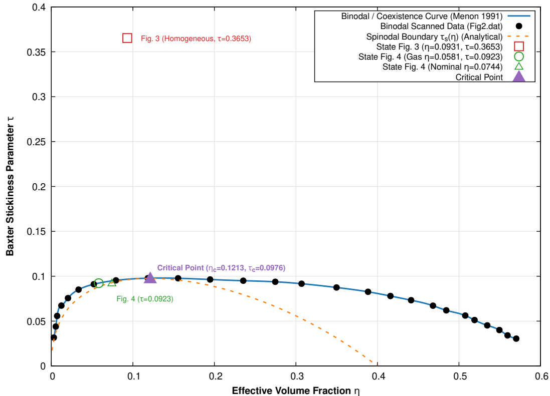
Menon et al. (1991) - Fig. 2: Adhesive Hard Sphere Phase Diagram
