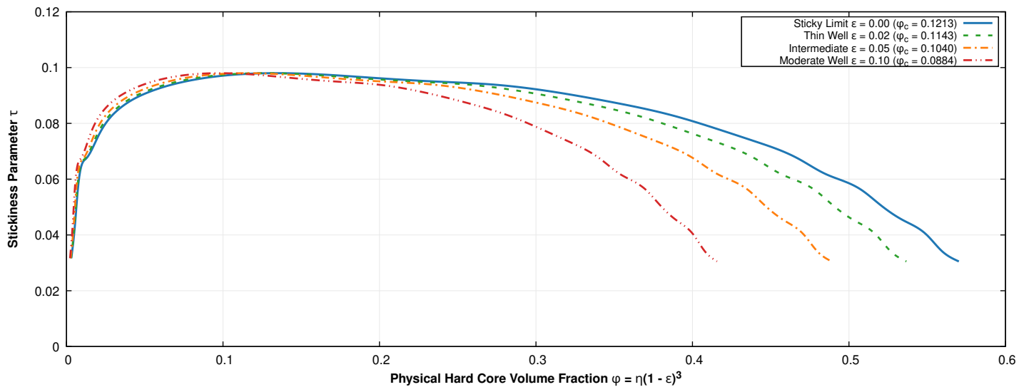
(a) Coexistence Boundary Evolution in (\varphi, \tau) Plane
