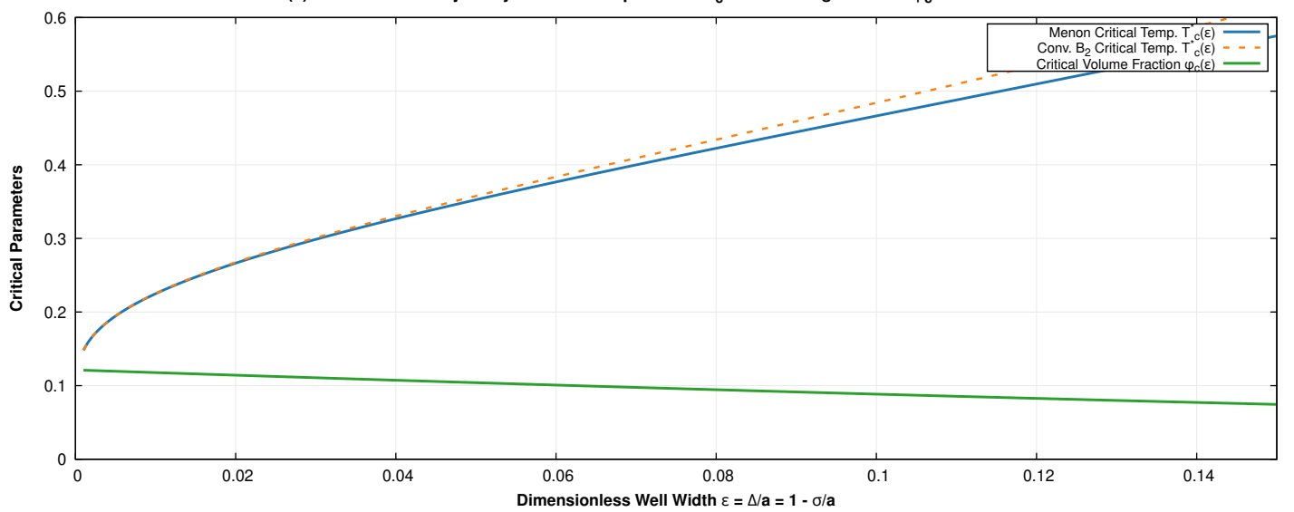
(c) Critical Point Trajectory: Critical Temperature T_c^* and Packing Fraction \varphi_c vs Well Width \varepsilon
