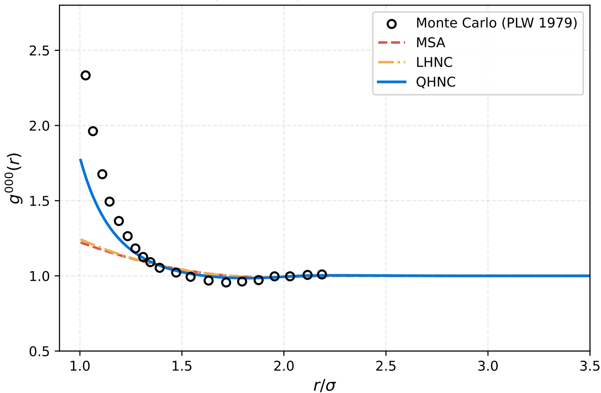
Patey et al. (1979) Fig. 1: Radial Distribution g^{000}(r)
