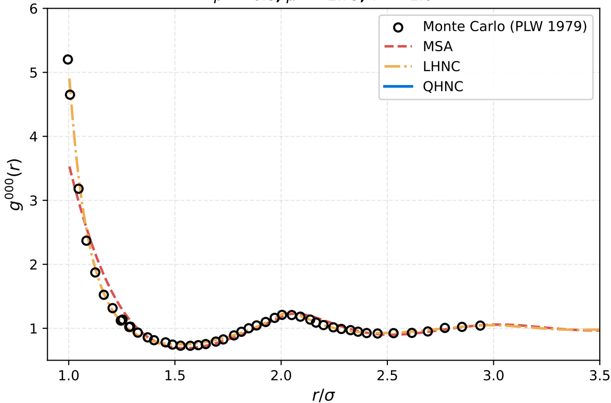
Patey et al. (1979) Fig. 4: Radial Distribution g^{000}(r)
