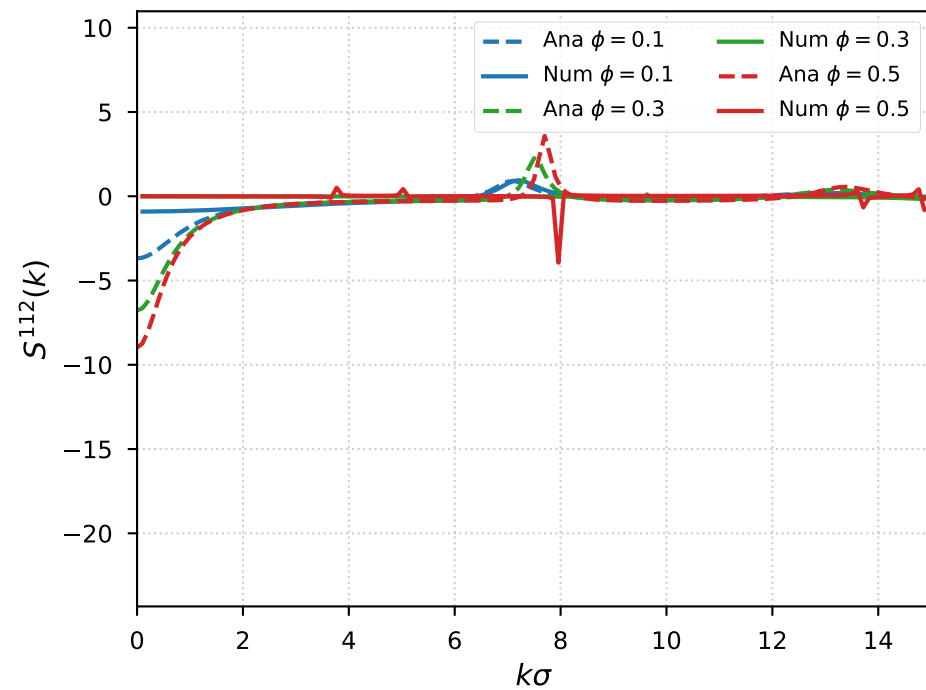
(d) S^{112}(k) at T^* = 0.01 (Direct Warm-Start)
