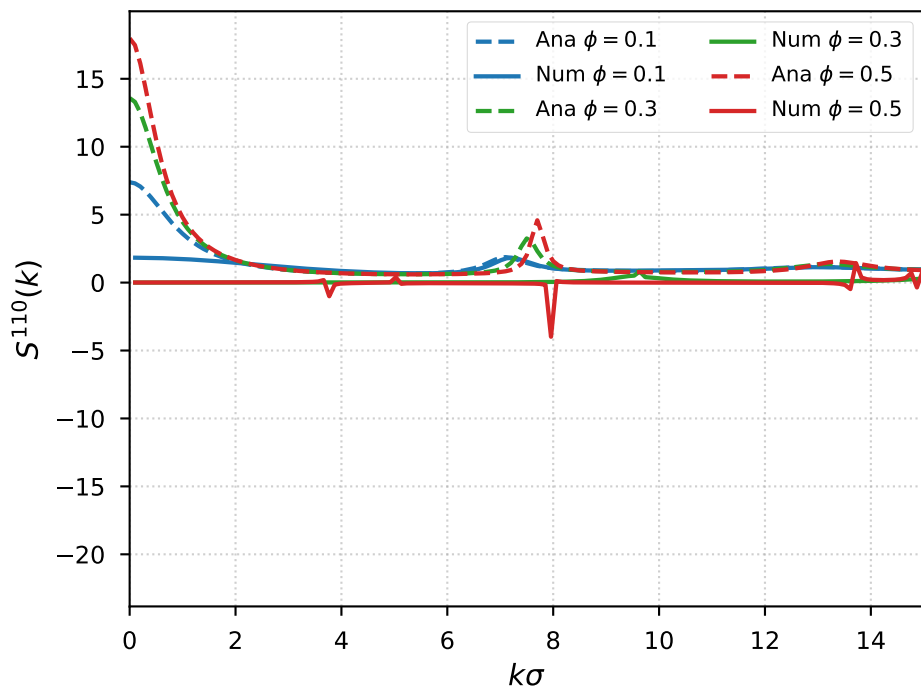
(c) S^{110}(k) at T^* = 0.01 (Direct Warm-Start)
