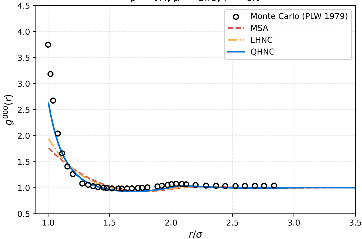
Patey et al. (1979) Fig. 2: Radial Distribution g^{000}(r)
