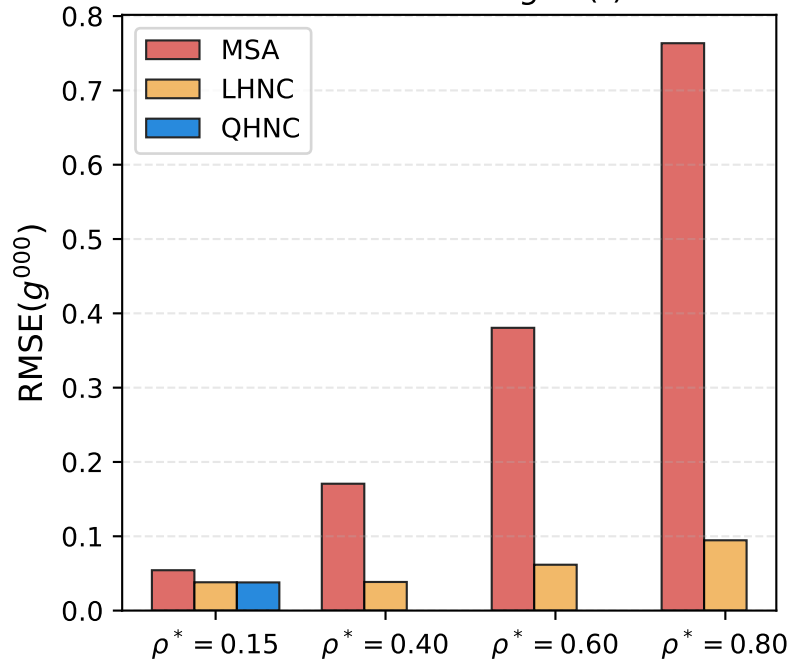
Radial Distribution g^{000}(r) Error
