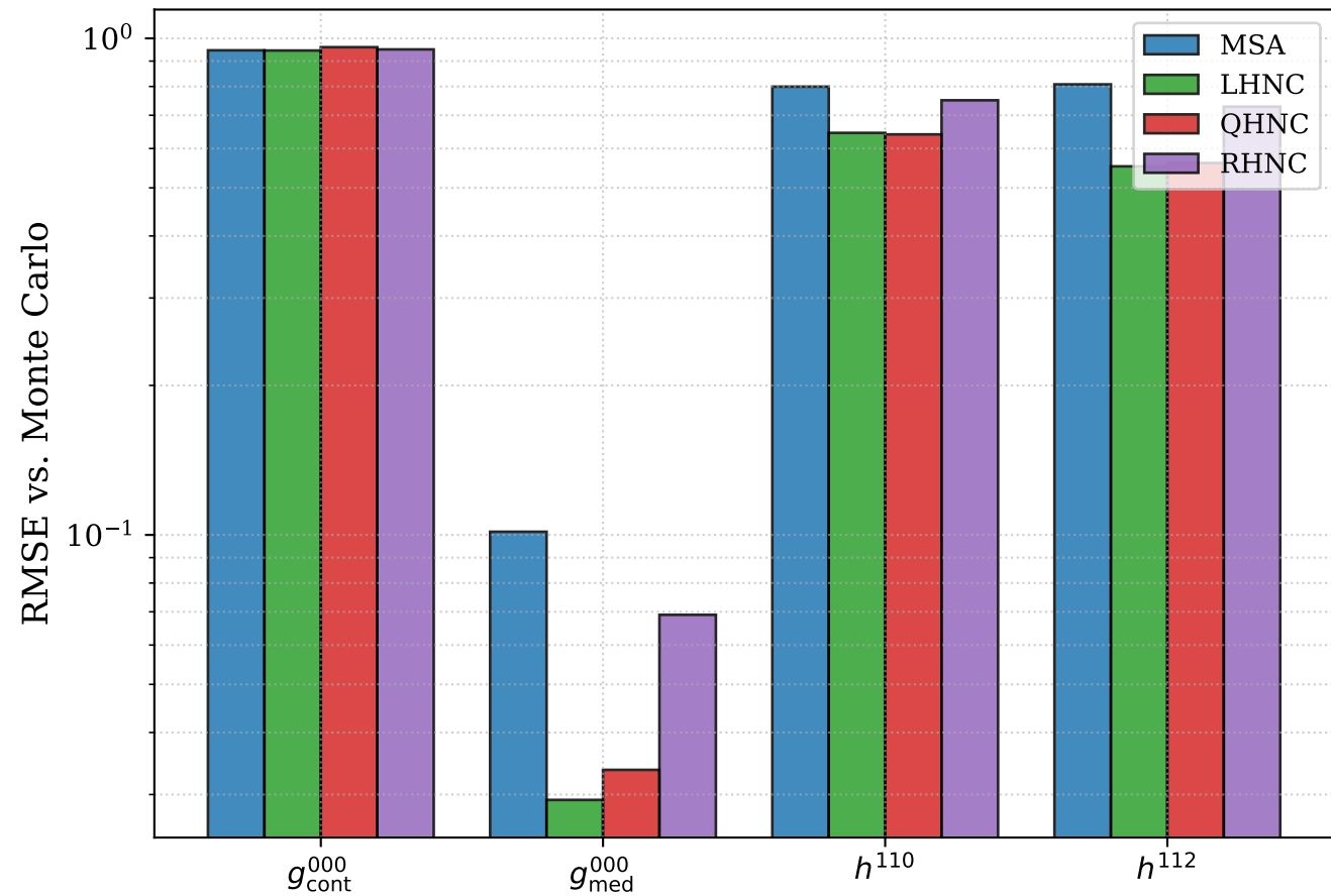
(b) State 2: \rho^* = 0.8, \mu^{*2} = 2.00 ( T^* = 0.5000 )
