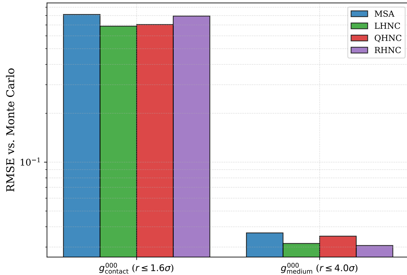
(a) State 1: \rho^* = 0.8, \mu^{*2} = 2.75 ( T^* = 0.3636 )
