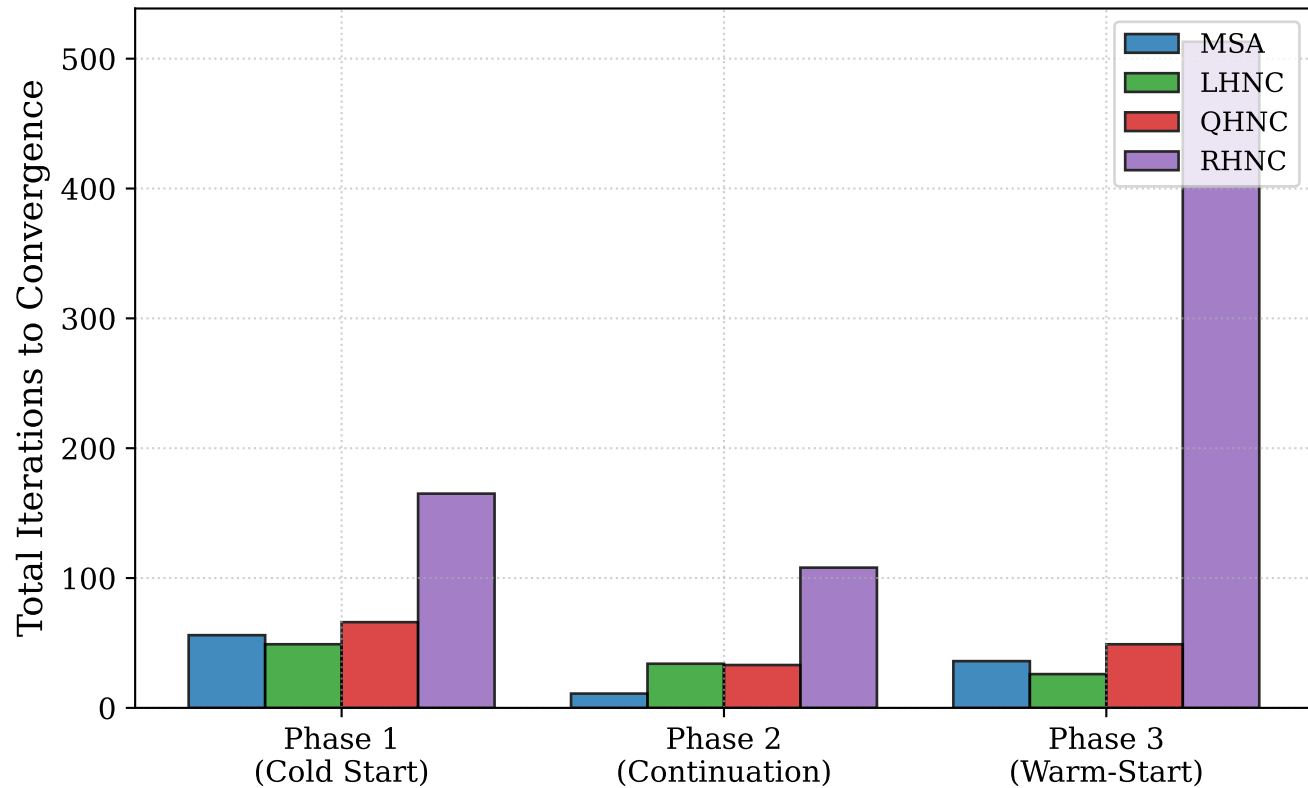
(b) State 2: \rho^* = 0.8, \mu^{*2} = 2.00 ( T^* = 0.5000 )
