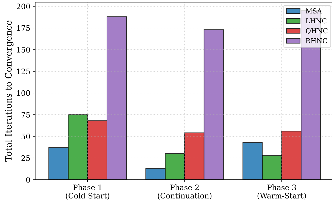
(a) State 1: \rho^* = 0.8, \mu^{*2} = 2.75 ( T^* = 0.3636 )
