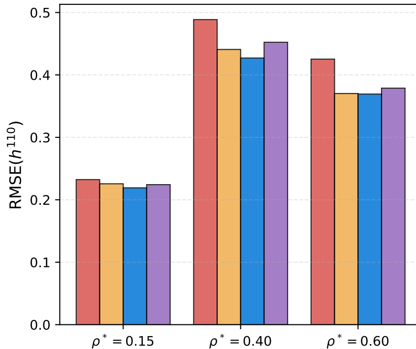
Dipolar Projection h^{110}(r) Error
