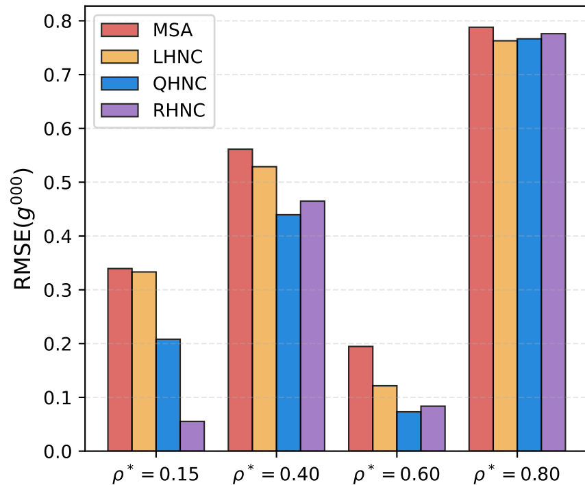
Radial Distribution g^{000}(r) Error
