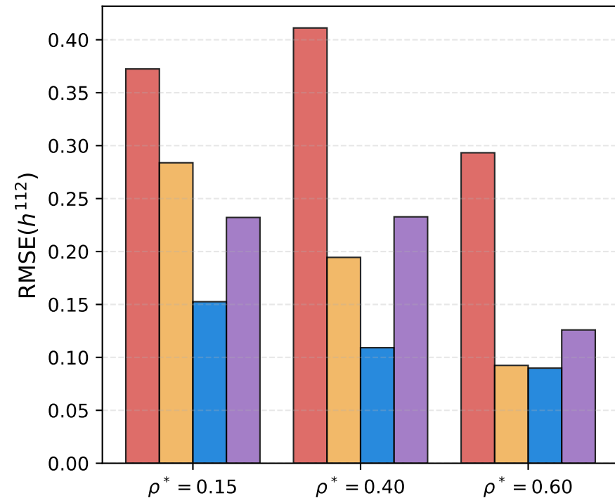
Anisotropic Projection h^{112}(r) Error
