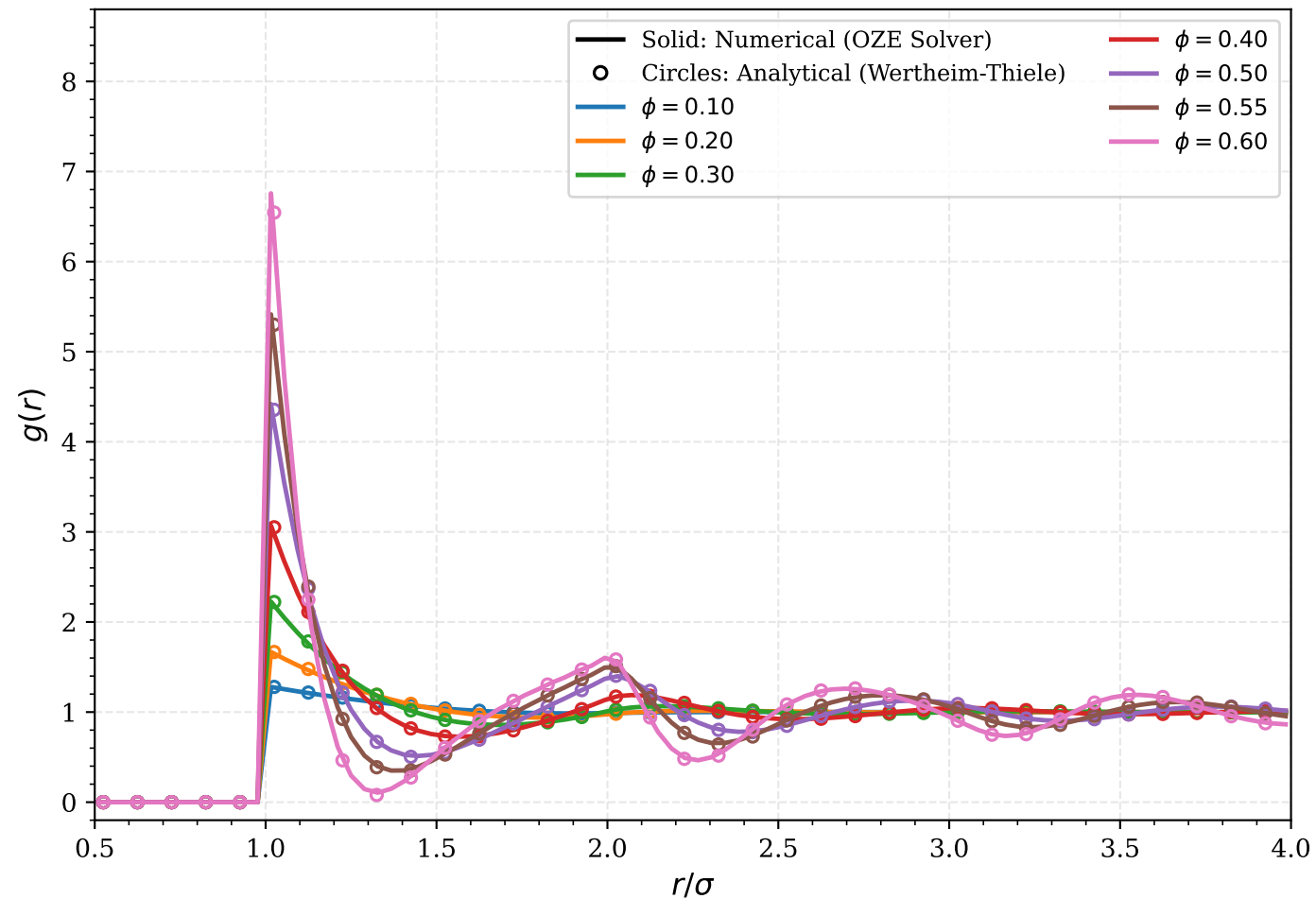
Percus-Yevick Hard Sphere Radial Distribution Function g(r)
