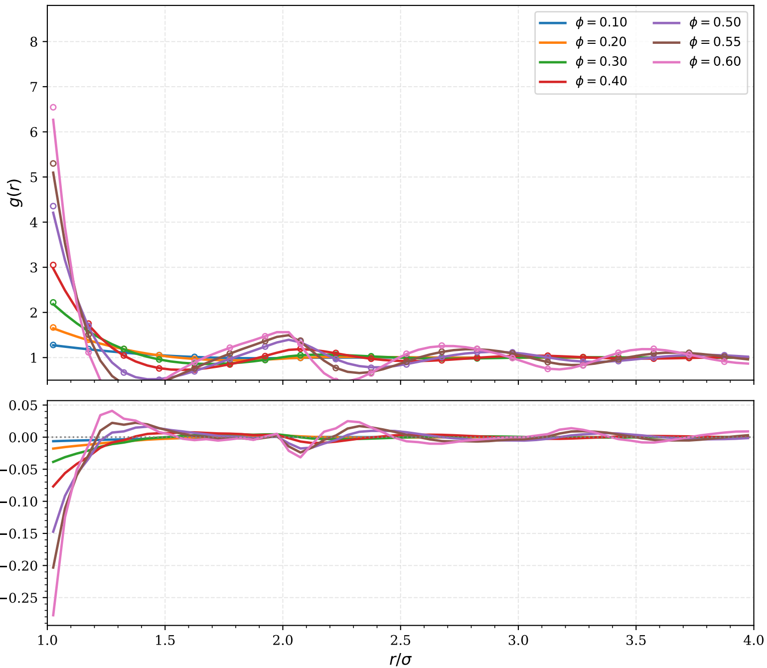
Fluid Region g(r) and Residual Deviations \Delta g(r) = g_{\text{num}}(r) - g_{\text{ana}}(r)
