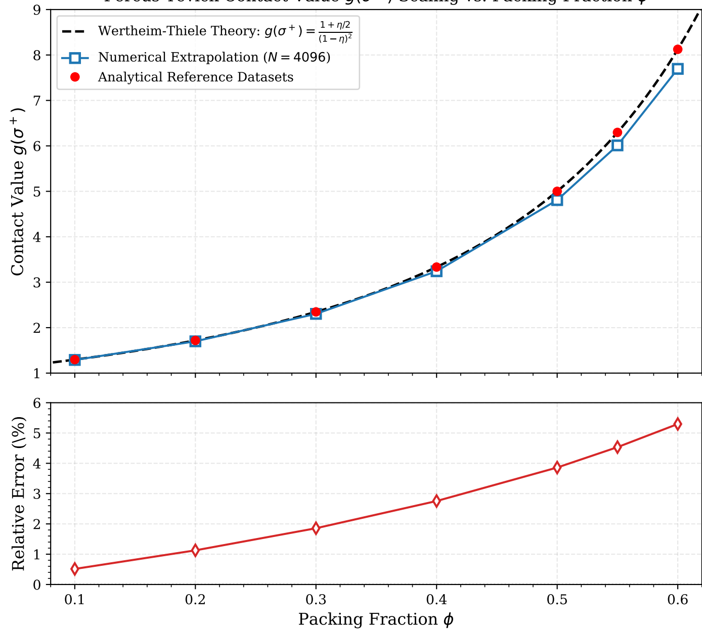
Percus-Yevick Contact Value g(\sigma^+) Scaling vs. Packing Fraction \phi
