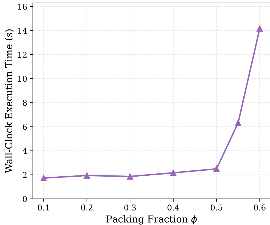
Solver Computational Performance
