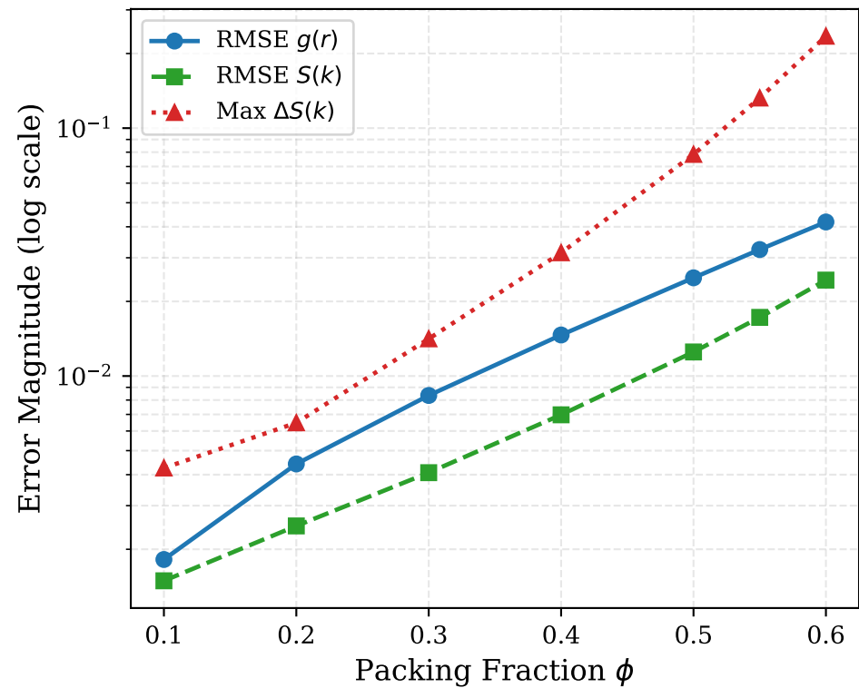
Numerical Error Metrics vs. \phi
