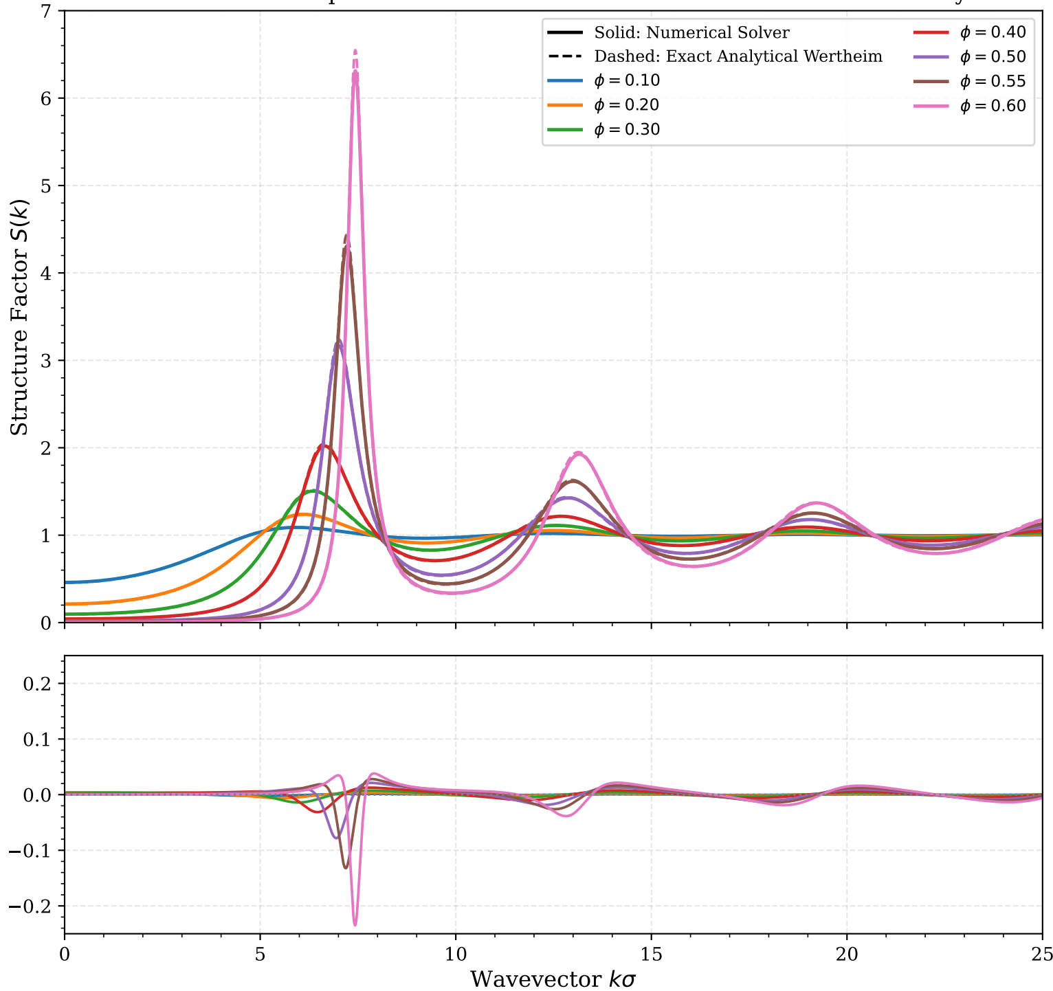
Percus-Yevick Hard Sphere Static Structure Factor: Numerical vs. Exact Analytical
