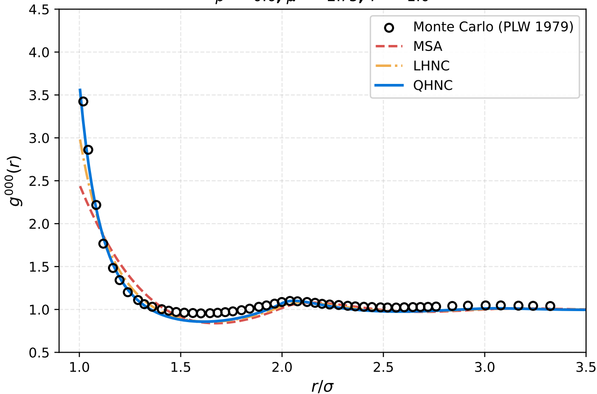
Patey et al. (1979) Fig. 3: Radial Distribution g^{000}(r)
