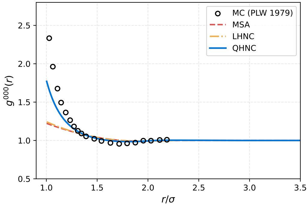
Panel (a): \rho^* = 0.15 , \mu^{*2} = 2.0 (PLW Fig. 1)
