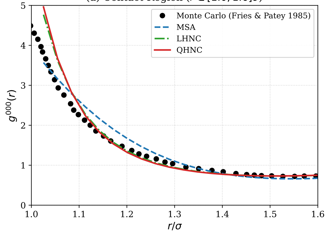
(a) Contact Region ( r \in [1.0, 1.6]\sigma )
