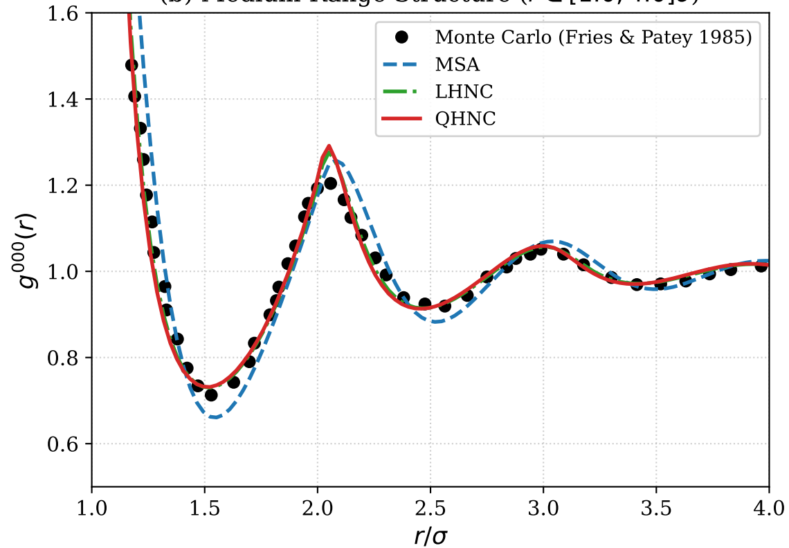
(b) Medium-Range Structure ( r \in [1.0, 4.0]\sigma )
