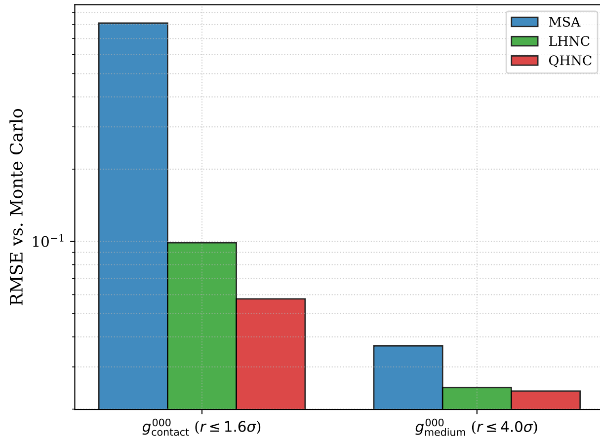
(a) State 1: \rho^* = 0.8, \mu^{*2} = 2.75 ( T^* = 0.3636 )
