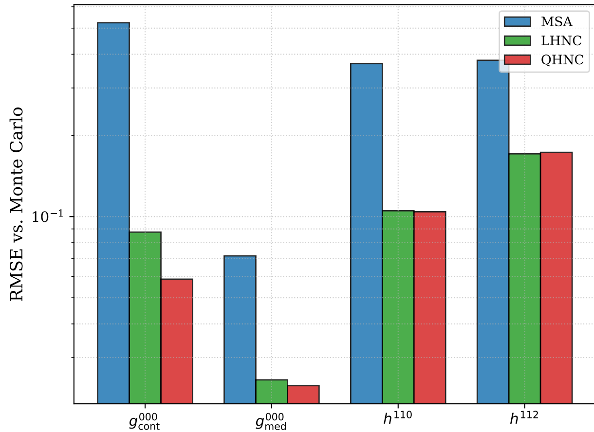
(b) State 2: \rho^* = 0.8, \mu^{*2} = 2.00 ( T^* = 0.5000 )
